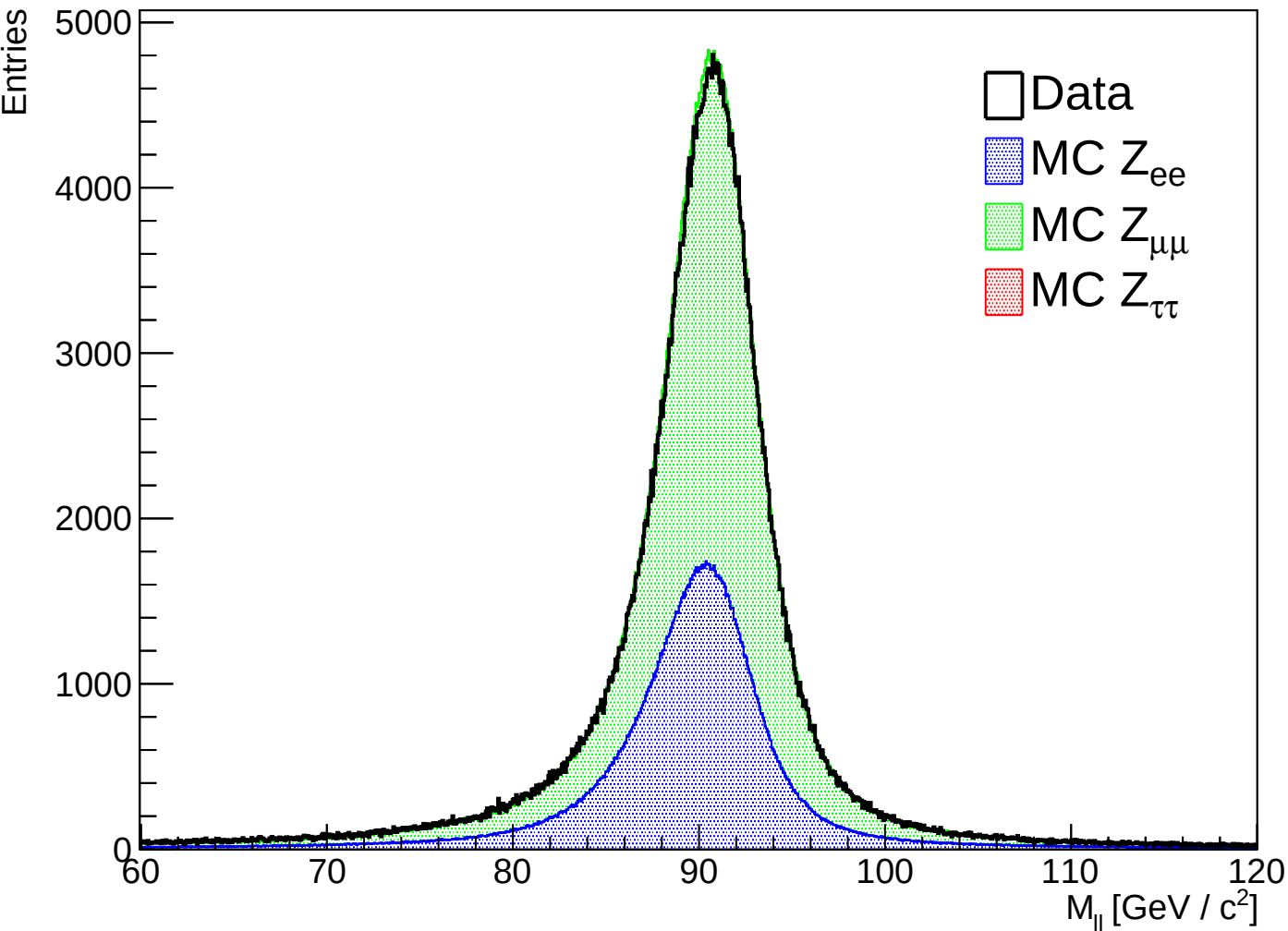
Comparison of Data and MC Calculations of Z Mass
